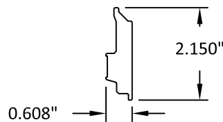
10 LOWER SASH BOTTOM RAIL, INT. WOOD
