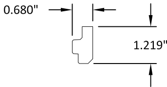
7 PARTING STOP, HEAD WOOD
