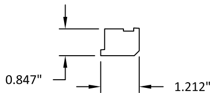
4 INTERIOR TRIM STOP, HEAD WOOD
