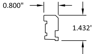
2 INTERIOR TRIM STOP, SILL WOOD
