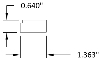
6 FILLER BLOCK, HEAD WOOD
