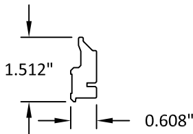
9 UPPER SASH CHECKRAIL, INT. WOOD
