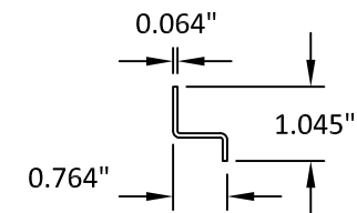
25 LOAD BRACKET CHECKRAIL GALV. STEEL (INTERLOCK)
