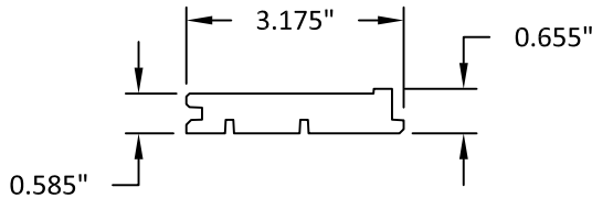
1 FRAME WOOD
