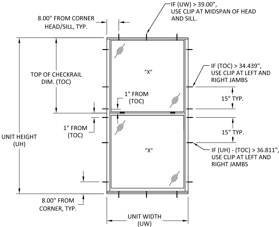
ANCHOR LAYOUT INSTALLATION CLIPS
