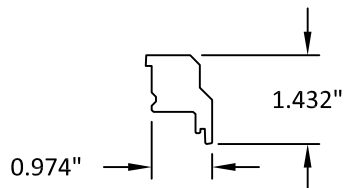
3 INTERIOR TRIM STOP, JAMB WOOD
