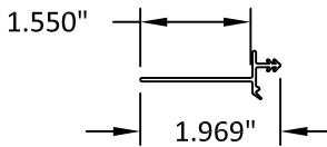
14 NAILING FLANGE RIGID PVC
