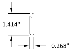
5 INTERIOR CENTER JAMB TRIM WOOD
