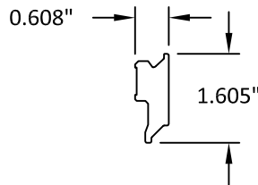
8 SASH RAIL/STILE, INT. WOOD
