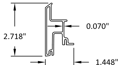
20 LOWER SASH BOTTOM RAIL, EXT. FIBERGLASS
